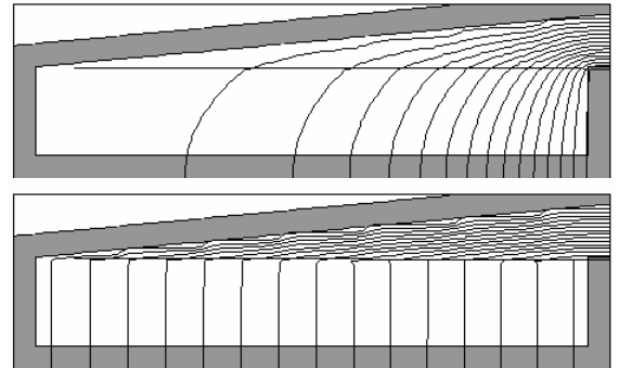
Fig. 4: Steady-state iso-potential contours (simulation). Above: liquid is a perfect dielectric. Below: liquid is a leaky dielectric.
