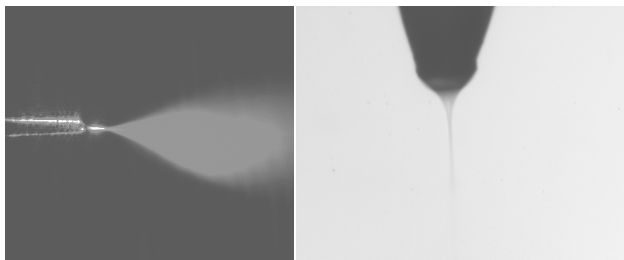
Fig. 11: Experiment images. Left is a micrograph showing an electro spray emitted from a gold-coated 60 \mu\text{m} diameter kapton tip. Right shows a Taylor cone that is formed at a capillary tip of diameter 32 \mu\text{m} . V_0=1600 \text{ V} , tip-to-counter-electrode distance is 1.5 \text{ mm} . The liquid is 1:1 acetonitrile:H 2 O (v/v), of conductivity 0.012 \text{ S/m} . The volumetric flow rate is 5 \text{ nanoliter per second} .
