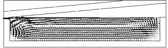
Fig. 3: Velocity plot (simulation). The density, viscosity, conductivity and relative permittivity of the liquid are 900 \text{ Kg/m}^3 , 0.055 \text{ Kg/m/s} , 8.05e-6 \text{ S/m} and 3 , respectively. The voltage is 10 \text{ KV} . a=0.022 \text{ m} , b=0.038 \text{ m} , and l=0.24 \text{ m} . Time frame shown is t=5.5 \text{ s} (steady state).
