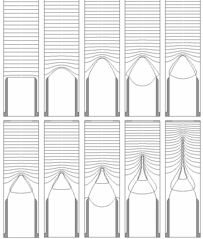
Fig. 7: Transient formation of a Taylor cone (simulation). The flow rate is 1423. The normalized times for the first three pictures are 0, 1022 and 2045; the following pictures are 68 apart. The Taylor cone shape (outlined by the curves originated from the tip of the nozzle) is plotted together with iso-potential lines.
