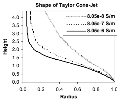
Fig. 10: Shape of the Taylor cone as a function of liquid electric conductivity (simulation).
