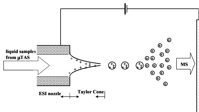
Fig. 1: Schematic of an ESI interface between a \mu fluidic unit and an MS.
