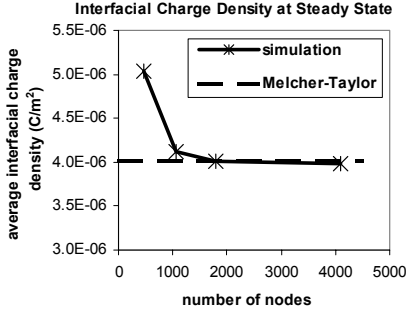
Fig. 5: Steady-state average interfacial charge density plotted versus mesh resolution. The dashed line is the Melcher-Taylor steady-state solution.
