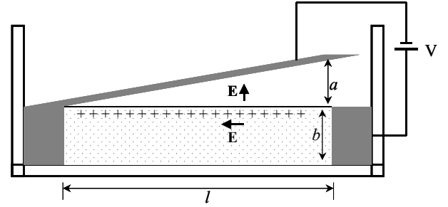
Fig. 2: Melcher-Taylor apparatus. The induced interfacial charge acts in concert with the electric field resulting in a counterclockwise cellular convection.
