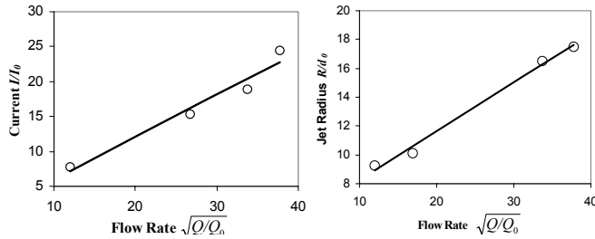
Fig. 9: Taylor cone radius and current as function of flow rate (simulation).
