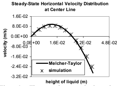
Fig. 6: The steady-state horizontal velocity distribution along the centerline. 1794 nodes are used.
