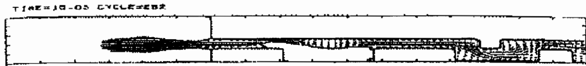
Figure 5. Channel Cross Section Showing Full Vapor Bubble Expansion
